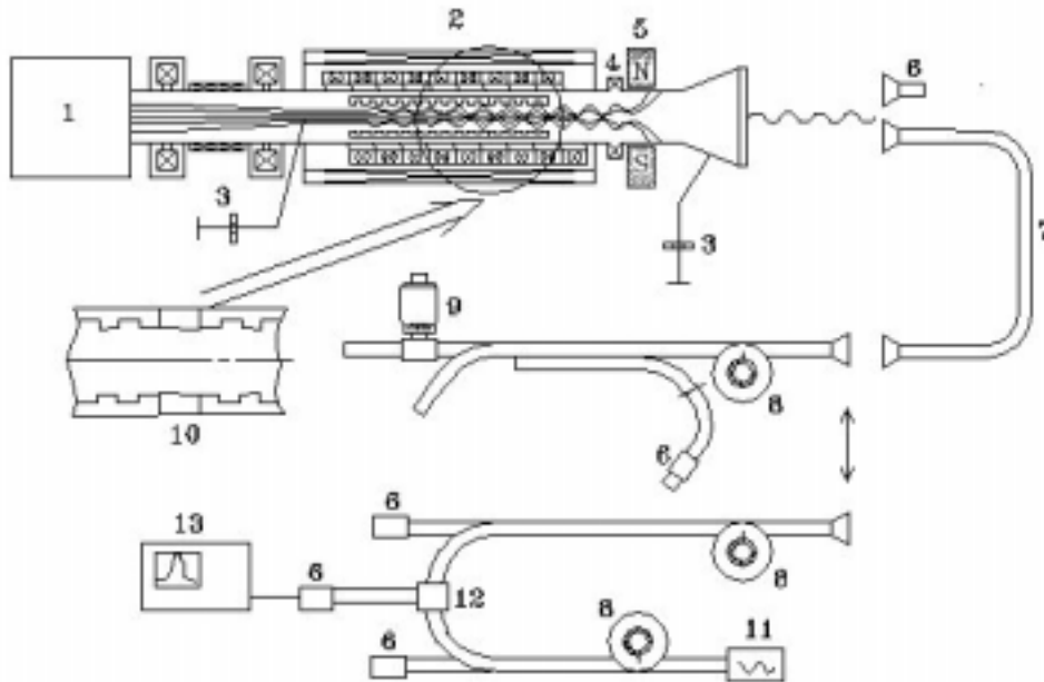
Fig. 2. Scheme of the experiment: 1) accelerator LIU-3000 as the electron beam injector; 2) FEM oscillator; 3) Rogowski coil; 4) isolator; 5) deflecting magnet; 6) calorimeter; 7) crystal detector of the microwave power; 8) attenuator; 9) wavemeter with the precise tuning of the resonant frequency; 10) insertion ring; 11) master oscillator; 12) RF frequency mixer; 13) digital oscilloscope.
