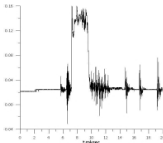
Fig. 3. Protons current.
