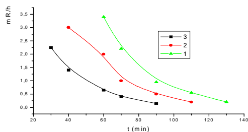
Fig. 2. The induced activity versus time after the beam turn-off.
