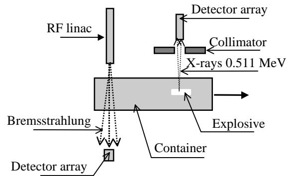
Fig.4. The container inspection system.
