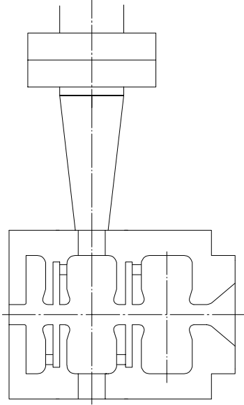
Fig. 2: Accelerating section
