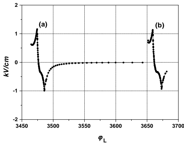
Fig. 6: Distribution of the microbunch space charge longitudinal electric field component: (a) – before the collimator, (b) – at the linac input
