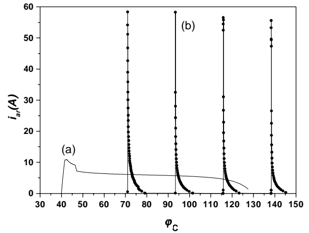
Fig. 3: Bunch current pulse at the tetrode output (input of the structure) (a);
