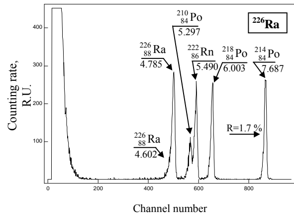
Fig. 2. Spectrum of ^{226}\text{Ra} alpha-particles obtained using a NPO «BIT» semiconductor detector of Si-PIN-PD type. Figures at the total absorption peaks denote the energy of alpha particles in MeV.
