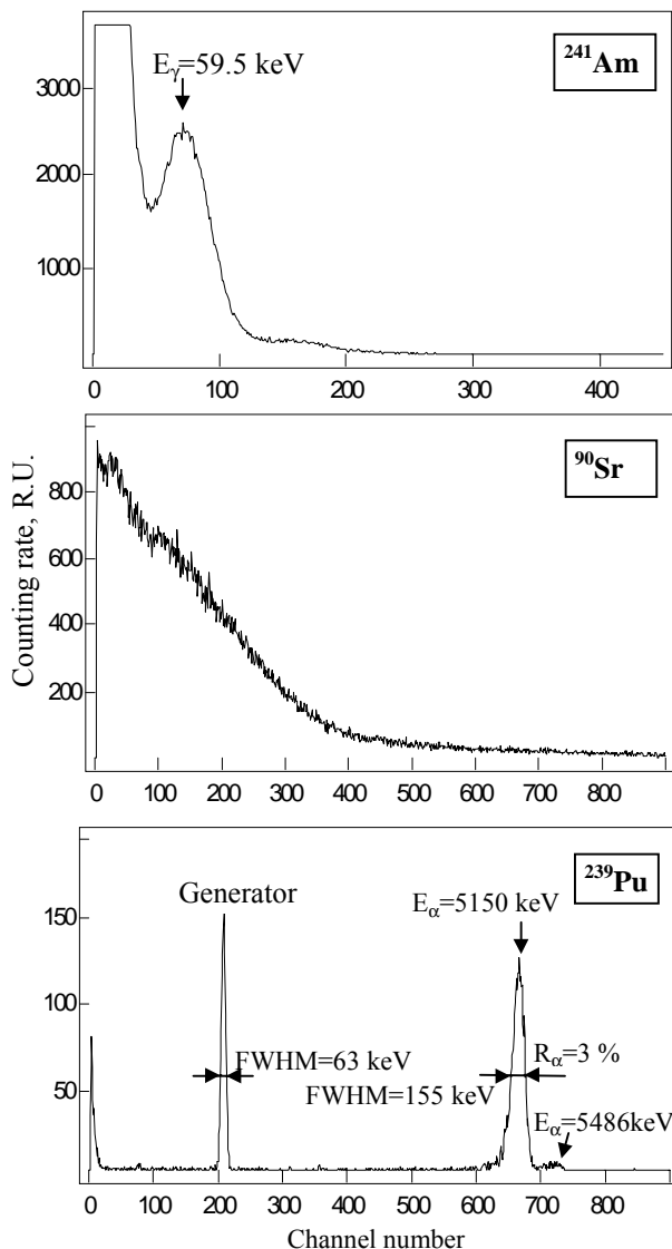
Fig. 4. Spectra of ^{241}\text{Am} gamma-quanta, ^{90}\text{Sr} beta-particles and ^{239}\text{Pu} alpha-particles obtained using a ZnSe(Te) based detector of 9x9x1 mm size and an S3590 Si-PIN-PD.
