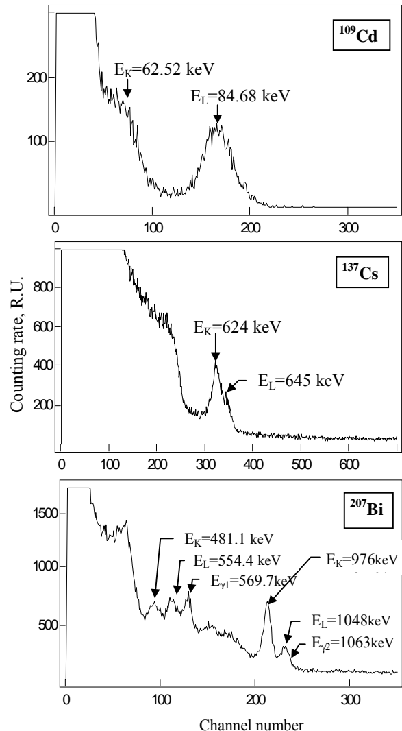
Fig. 3. Spectra of ^{109}\text{Cd} ( E_\gamma=85.03 \text{ keV} ), ^{137}\text{Cs} ( E_\gamma=662 \text{ keV} ), ^{207}\text{Bi} ( E_{\gamma 1}=569.7 \text{ keV} and E_{\gamma 2}=1063 \text{ keV} ) internal conversion electrons obtained using a ZnSe(Te)-based detector of 9 \times 9 \times 1 \text{ mm}^3 size and an S3590 Si-PIN-PD.
