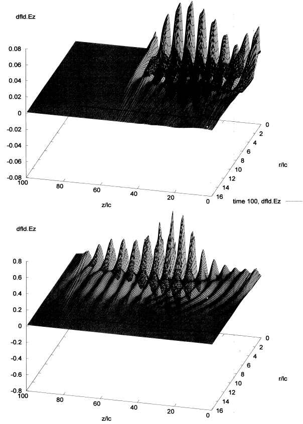
Fig. 1. 2-D distribution of the longitudinal electric field E_z for the instances of time t = 60\omega_{pe}^{-1} and t = 100\omega_{pe}^{-1} .
