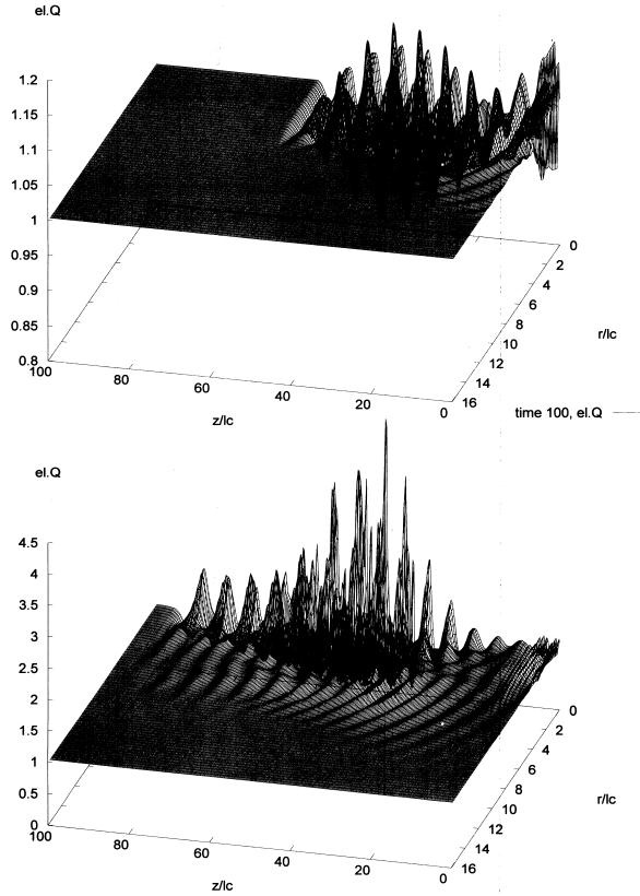
Fig. 2. 2-D distribution of the plasma electron density el.Q for the instances of time t = 60\omega_{pe}^{-1} and t = 100\omega_{pe}^{-1} .
