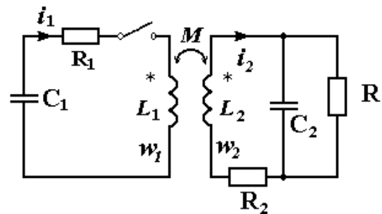
Fig. 1. Electrical schematic of the Tesla transformer.
