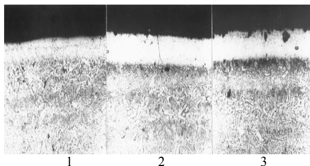
Fig. 1. Cross-sections of metallographic samples of alloyed steel, undergone to single irradiation with a high-energy beam of 300 keV energy.
