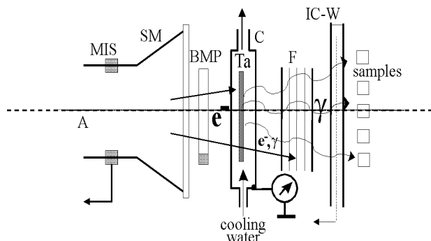
Fig. 1. Schematic of the radiation forming and diagnostics devices.
