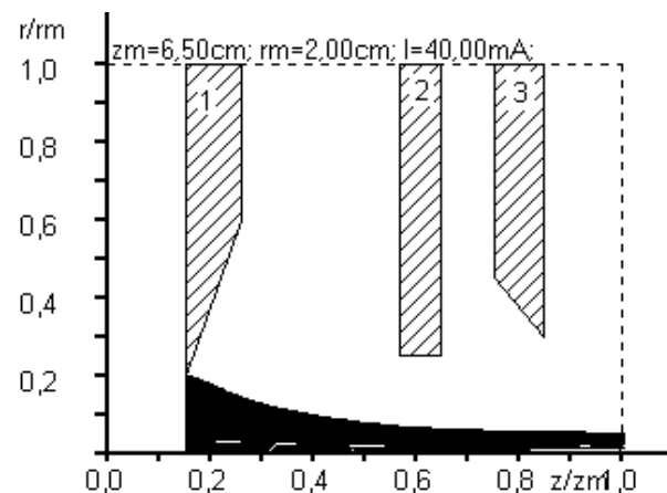
Fig. 1. Deuteron trajectories for the beam current I=40\text{mA} .
