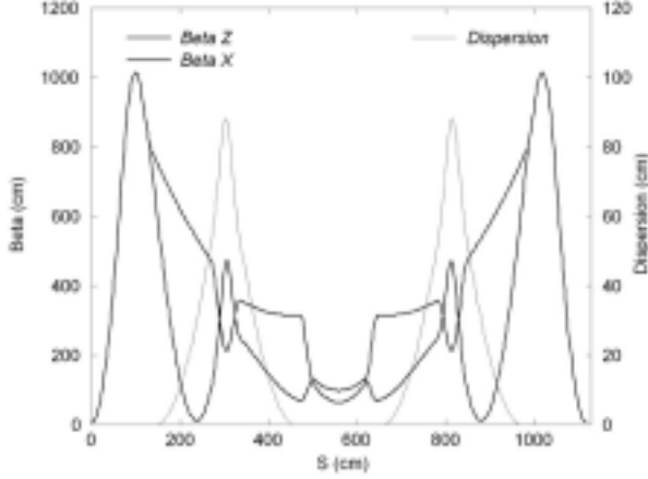
Fig. 2. Half period lattice functions. S=0 corresponds to IP.
