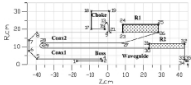
Fig. 3. Cross-section of the cavity. The locations of HOM.
