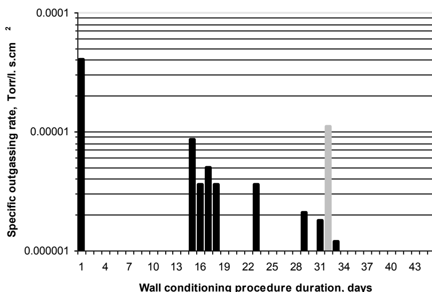
Fig.1. Stainless steel probe outgassing rate (250°C) on the time of U-2M wall conditioning process.
