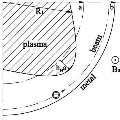
Fig. 1. Schematic of the plasma-beam system
