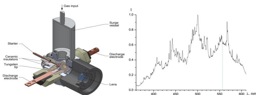
Fig. 1. The design of a pulsed light source
