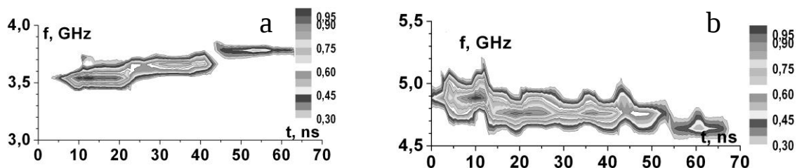
Fig. 1 Frequency tuning in G-band, 50-MW pulse: a – rise, b - reduction
