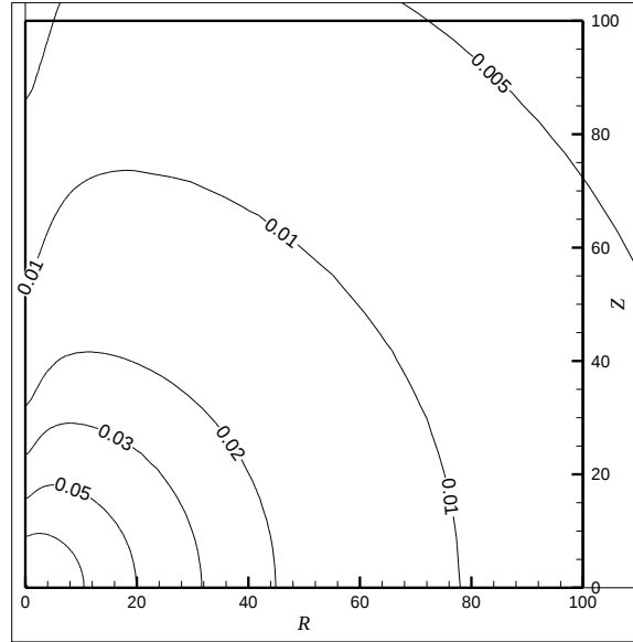
Fig.1. Potential (-e\varphi/T) lines in weakly-ionized magnetoactive plasma with spherical grain. R=r/r_D , Z=z/r_D
