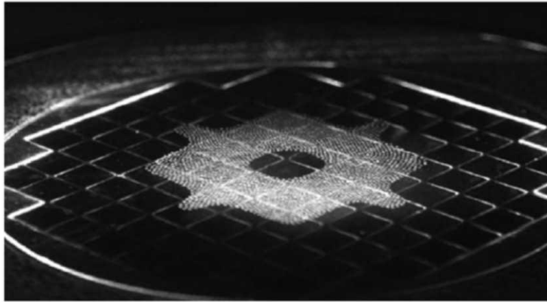
Fig.1: A two-dimensional cloud of mono-disperse dust micro-particles ( 10^{\mu\text{m}} ) is trapped in a plasma sheath in front of the adaptive electrode in an rf-plasma. The electrode is segmented, allowing for manipulation of the trapped micro-particles in real time.
