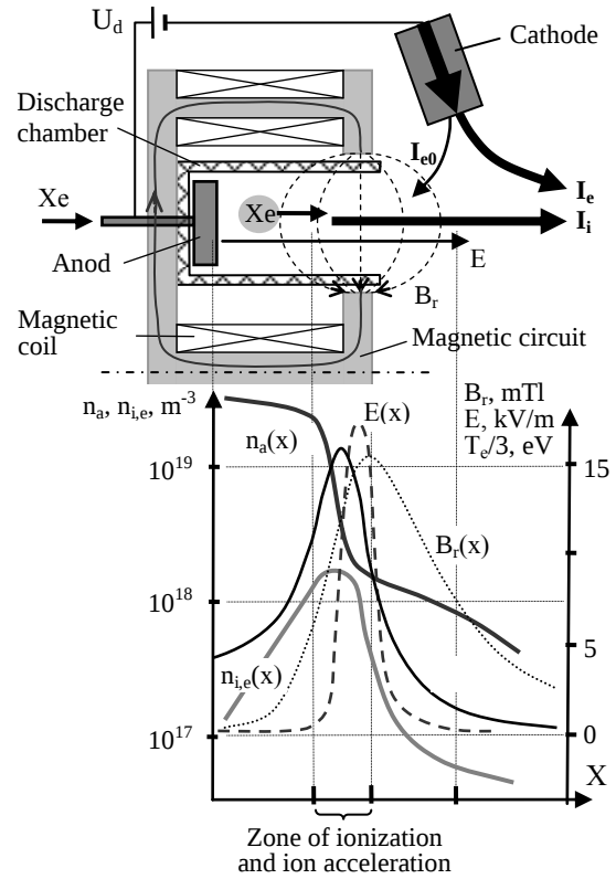
Fig. 1. Plasma parameters distribution in the discharge interval.
