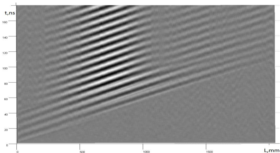
Fig.1 Space-time distribution of the E_z electric field component near the system axis
