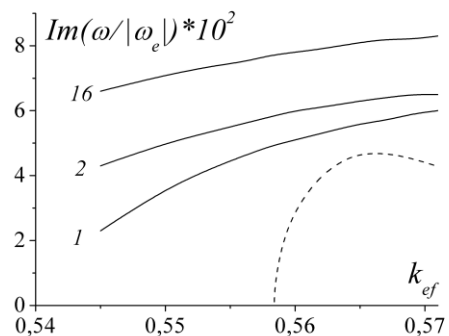
Fig. 2. HF ASW growth rates vs k_{ef} = |m|c/(\Omega_e a)
