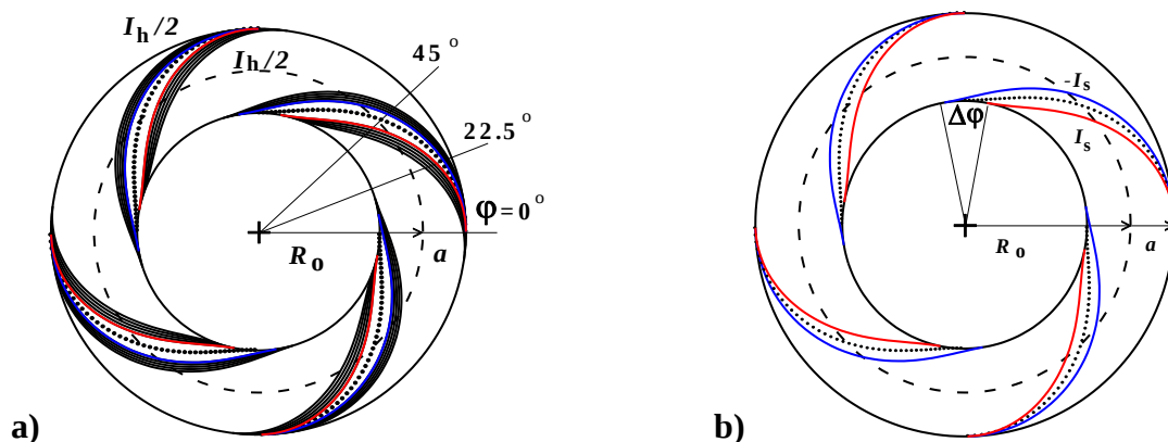
Fig.1. Top view of internal split-type main helical coils of the calculation model (a) and, separately, the internal split-type SCW (b), \Delta\varphi is the toroidal angle of splitting. The helical base lines are shown as dotted lines. The toroidal azimuths of poloidal cross-sections are indicated. The additional magnetic field coils are not shown.
