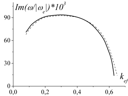
Fig. LF ASW growth rates vs k_{ef} = |m|c/(\Omega_e a)
