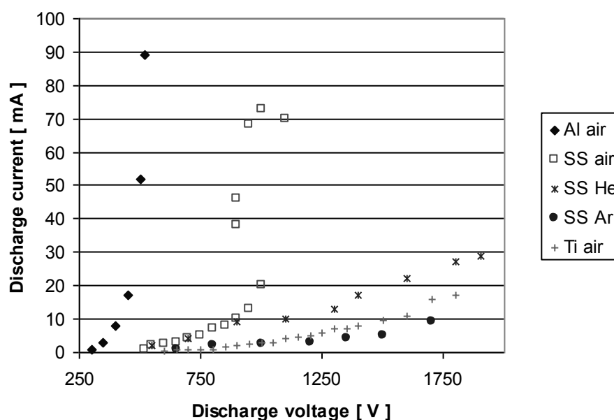
Fig. 1. Current-voltage characteristics of mirror Penning discharges.
