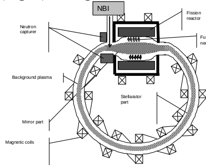
Fig. 1. Sketch of the fission-fusion hybrid.
